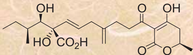
Alternaric acid
